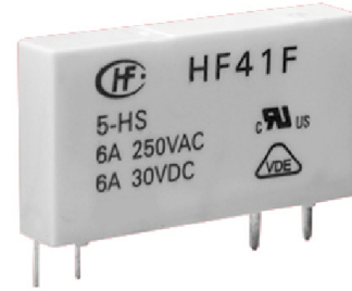
Relay HF41F
